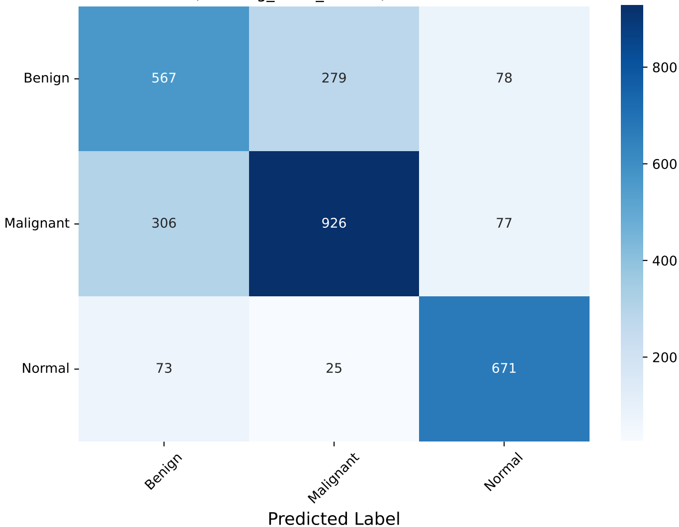
Fused Model (stacking_meta_learner) -- Test Confusion Matrix
